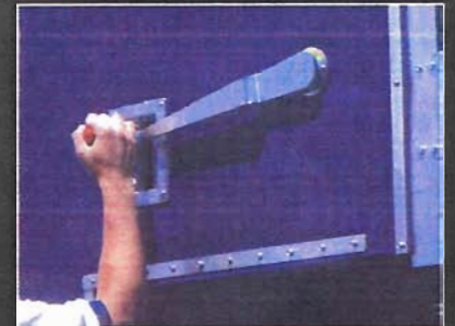
Rear-Locking System
